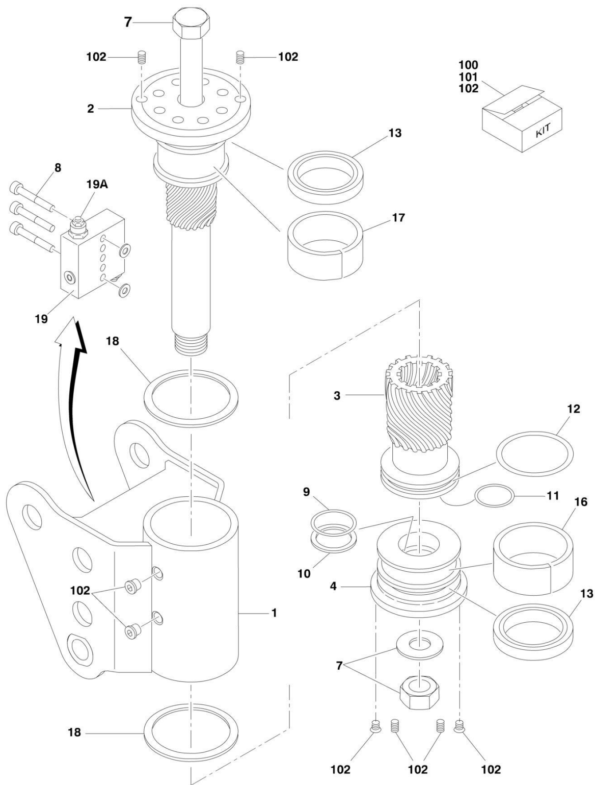
FIGURE 3-8. JIB SWING ROTATOR ASSEMBLY (E300AJP ONLY) (Prior to SN 0300064982)
